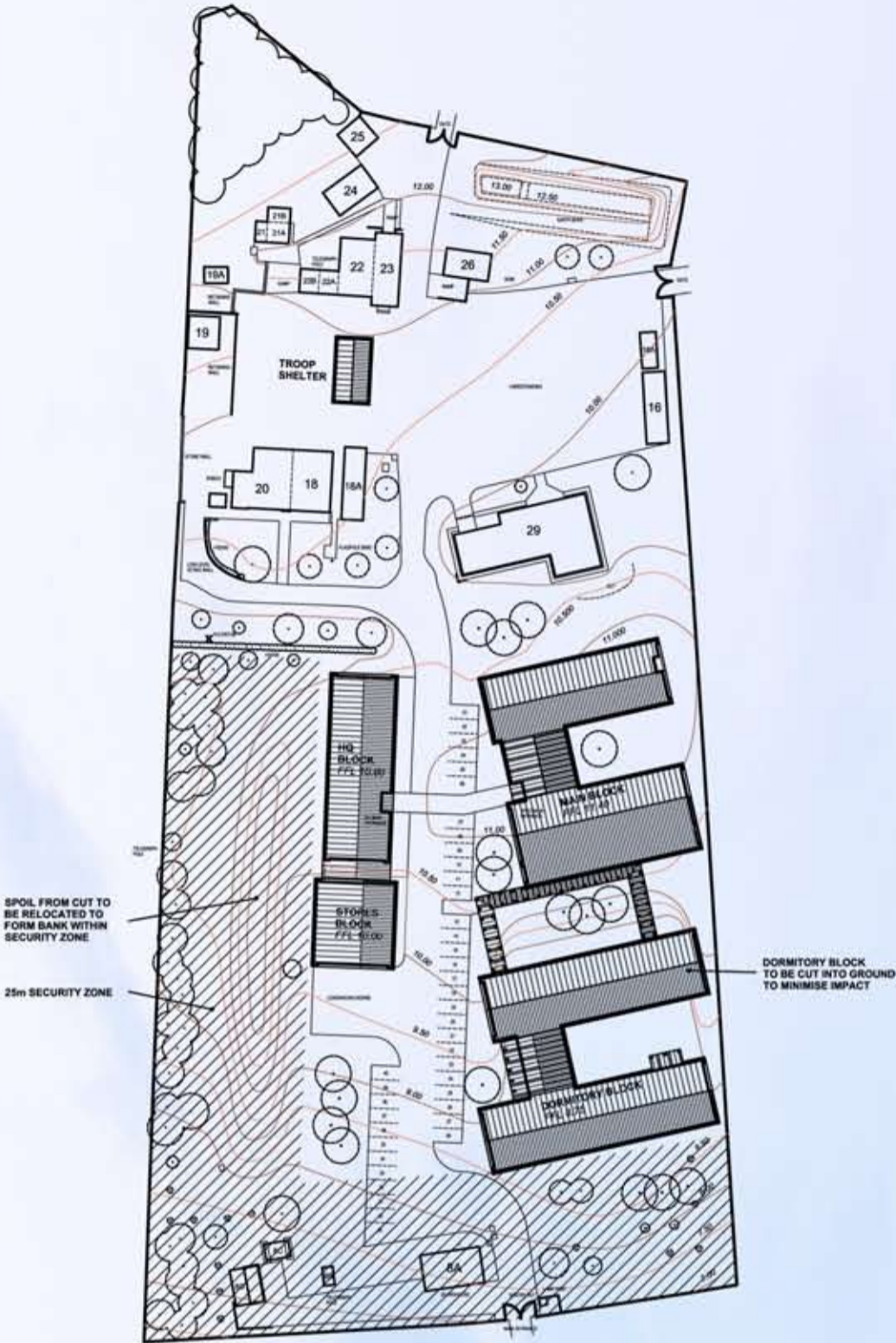
SITE PLAN AS PROPOSED
