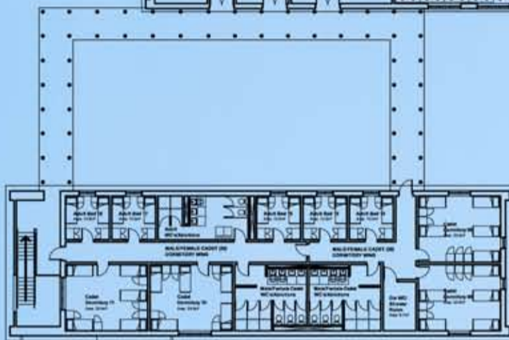
DORMITORY BUILDING (North Wing) UPPER GROUND FLOOR PLAN GIA: 318m 2
