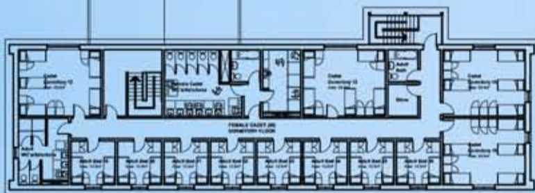
DORMITORY BUILDING (South Wing) UPPER GROUND FLOOR PLAN GIA: 370m 2
